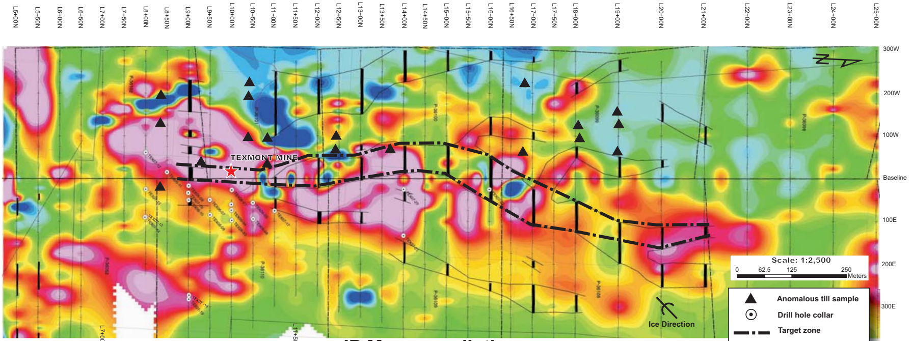
IP Mag compilation map
